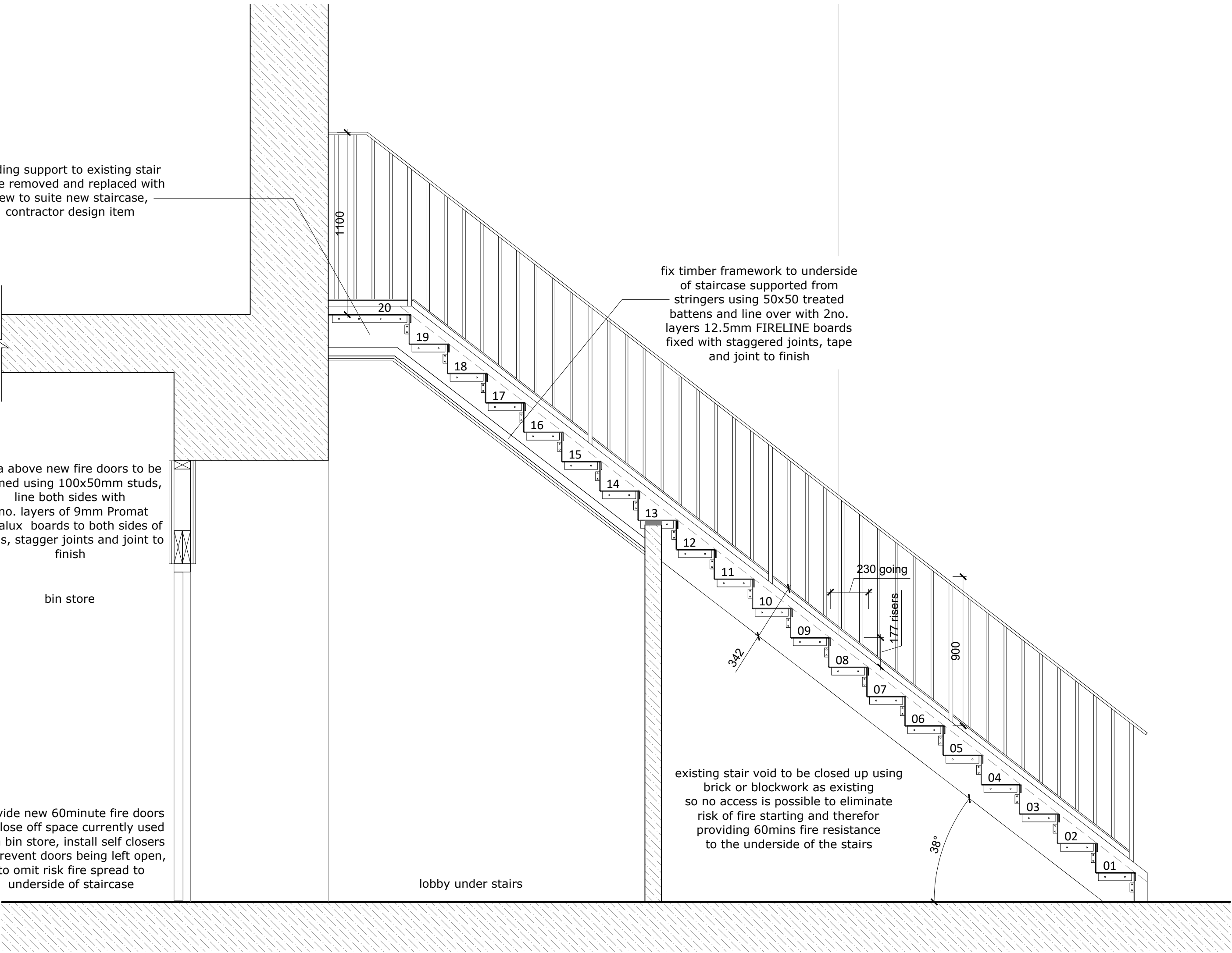
Proposed Section B-B 1:20 @ A1
