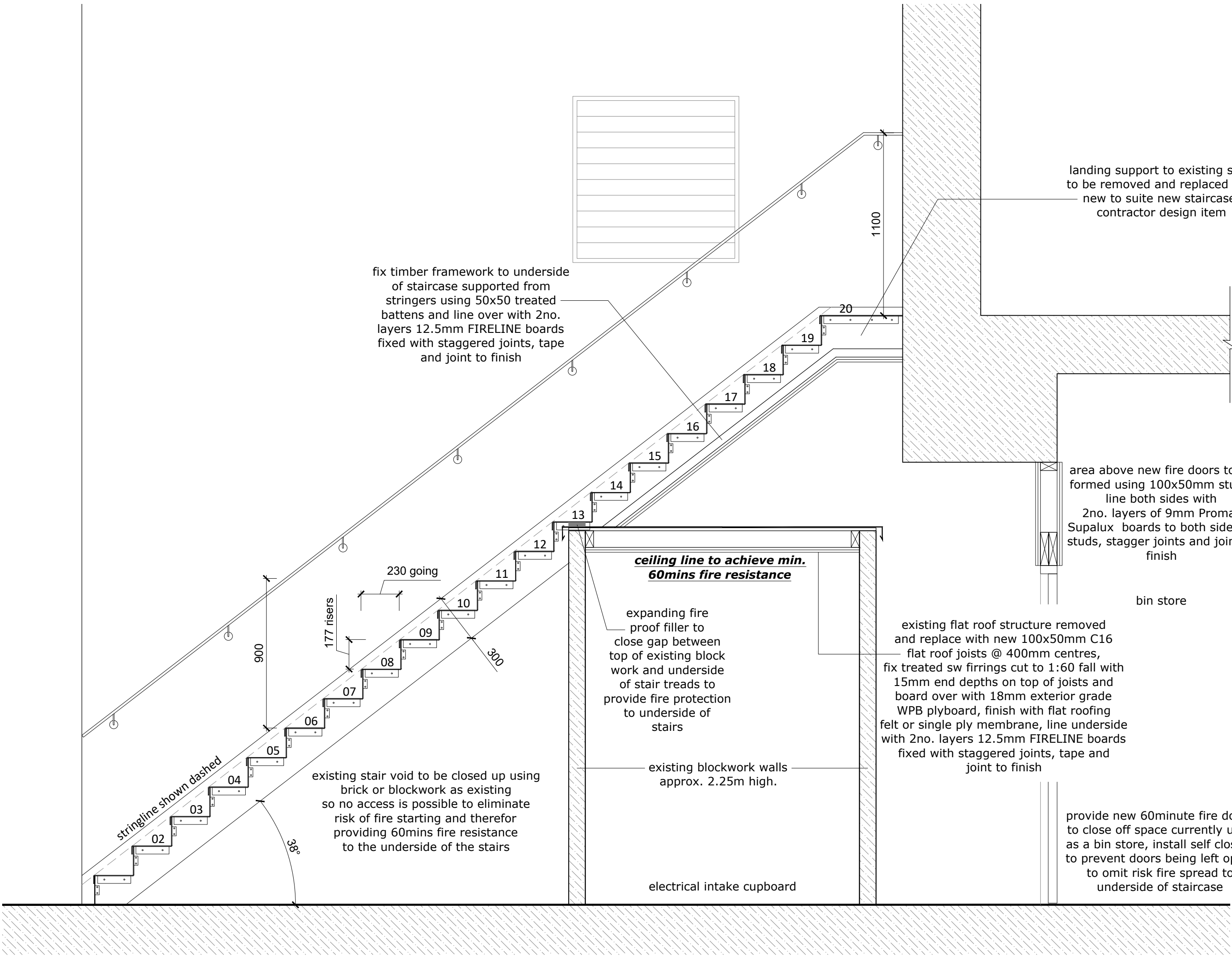
Proposed Section A-A 1:20 @ A1
